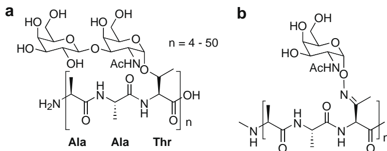
Figure 1. (a) Structure of naturally occurring AFGPs; (b) proposed AFGP mimic.
